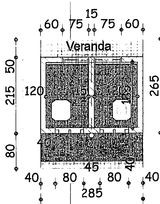
PLAN DISTRIBUTION
