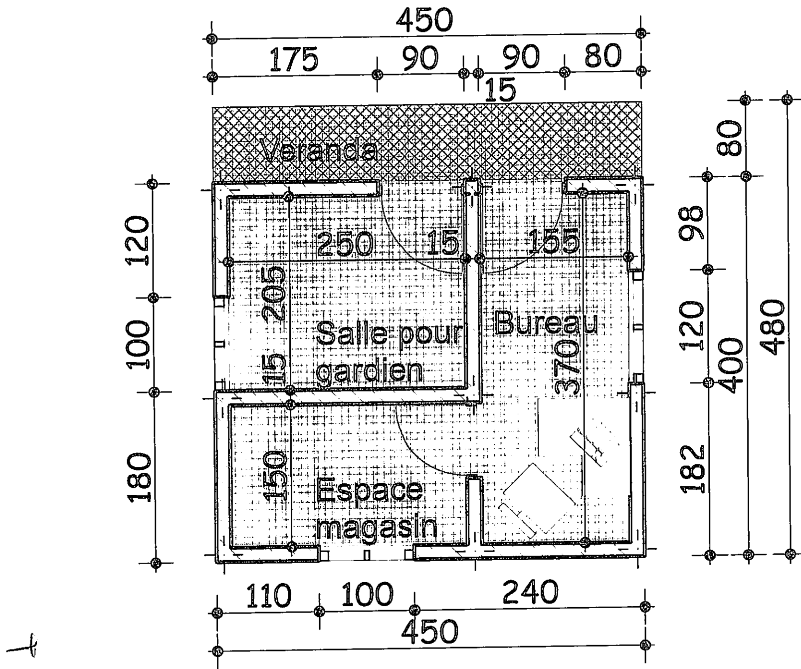
Plan distribution du local-centre
